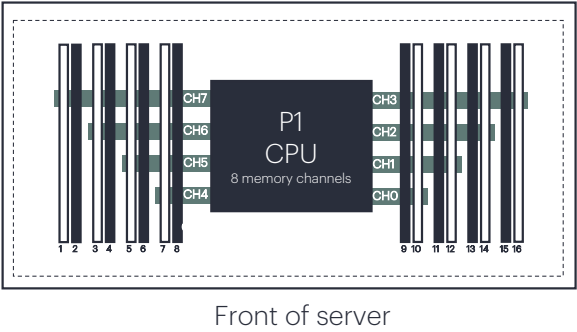
Figure 7. DIMM slot locations in DL320/DL340 Gen12 servers with 6th Gen Intel Xeon
