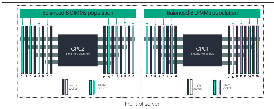
Figure 3. Example of a memory configuration that is balanced across processors
