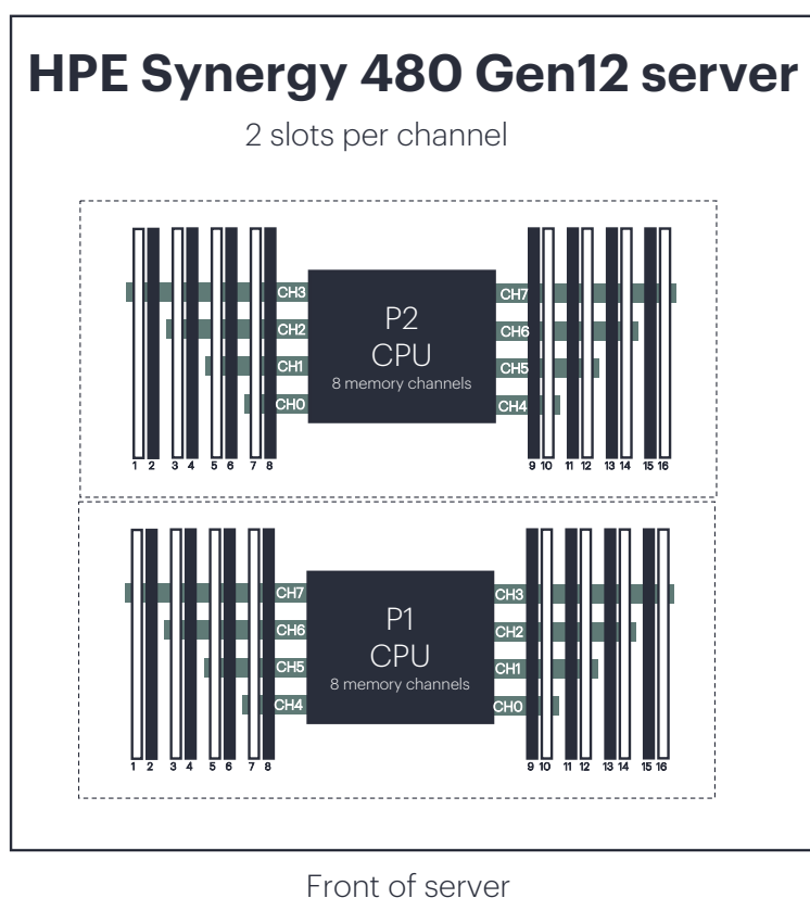
Figure 6. DIMM slot locations for 480 Gen12 servers with 6th Gen Intel Xeon compute modules (P1 and P2 are rotated.)
