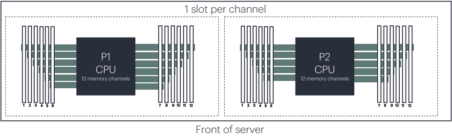
Figure 8. DIMM slot locations in XD230 servers with 6th Gen Intel Xeon
