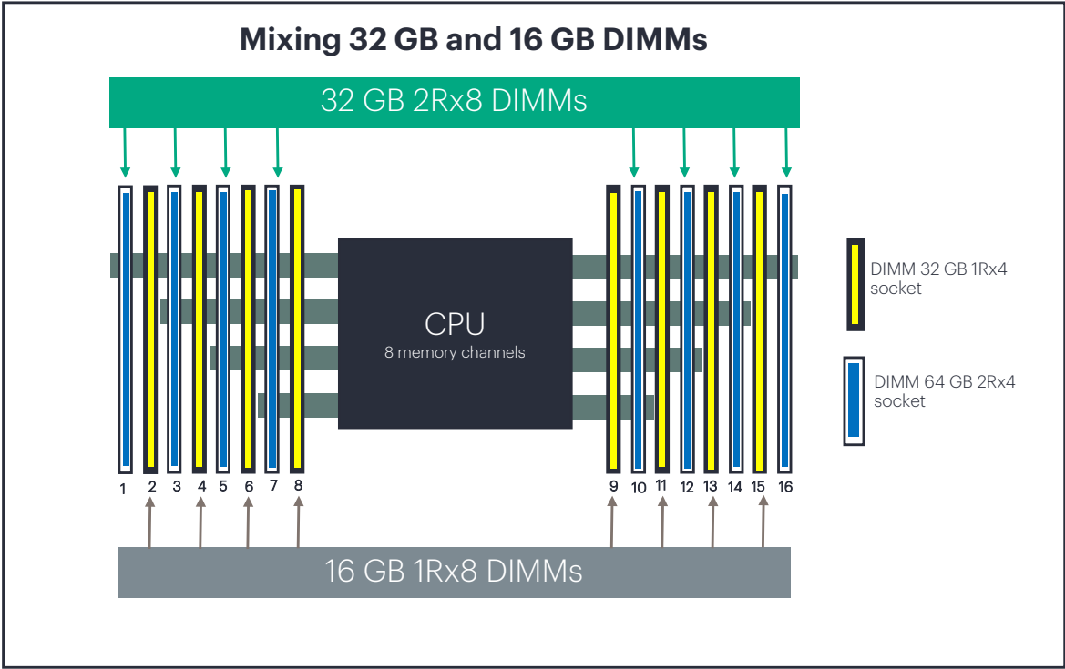
Figure 9. Mixing HPE DDR5 Smart Memory 32 GB 2Rx8 and 16 GB 1Rx8 mixed configuration
