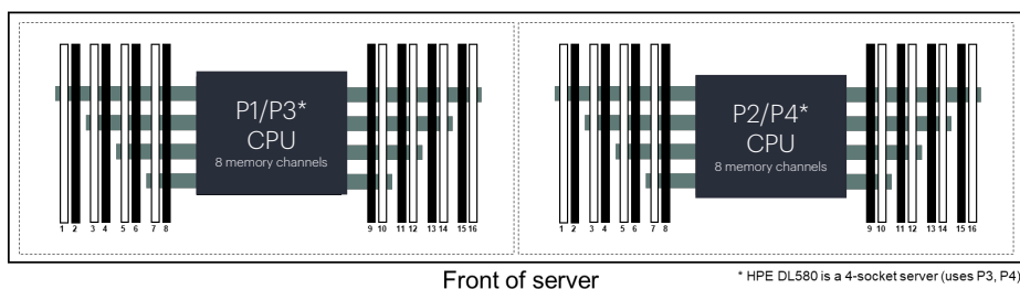
Figure 5. DIMM slot locations in DL380a/DL580 Gen12 servers with 6th Gen Intel Xeon
