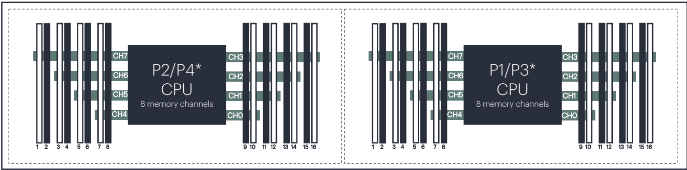
Figure 4. DIMM slot locations in DL360/DL380/ML350 Gen12 servers with 6th Gen Intel Xeon
