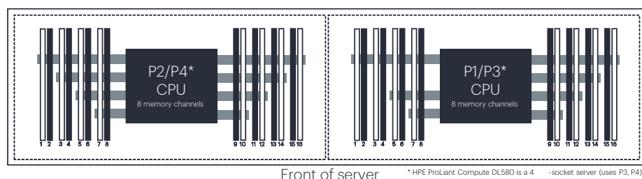
Figure 1. 32 DIMM slot locations in DL360/DL380/ML350 Gen12 servers with 6th Gen Intel Xeon
