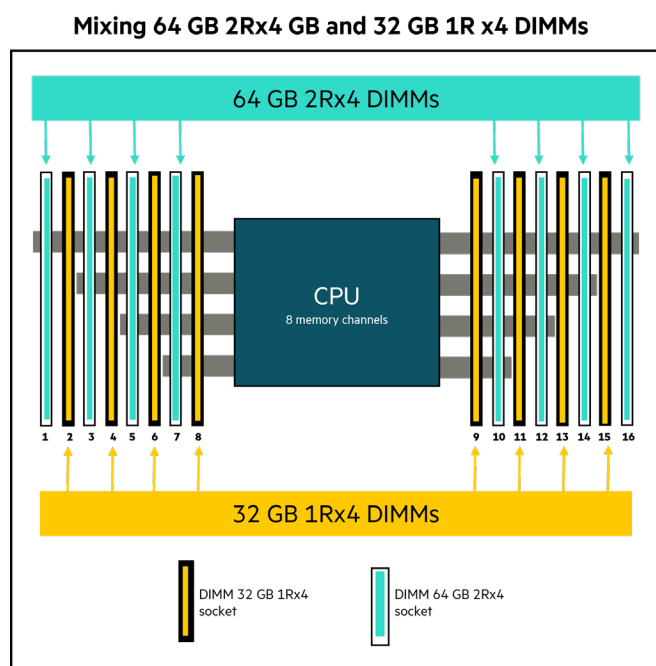
Figure 11. Mixing HPE SmartMemory 64 GB 2Rx4 and 32 GB 1Rx4 mixed configuration
