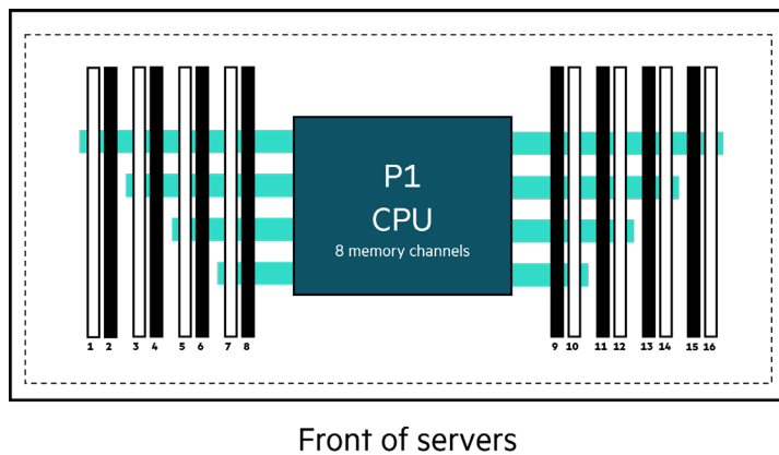
Figure 7. DIMM slot locations in HPE ProLiant DL320/ML110 Gen11 (5th Intel Xeon) Servers
