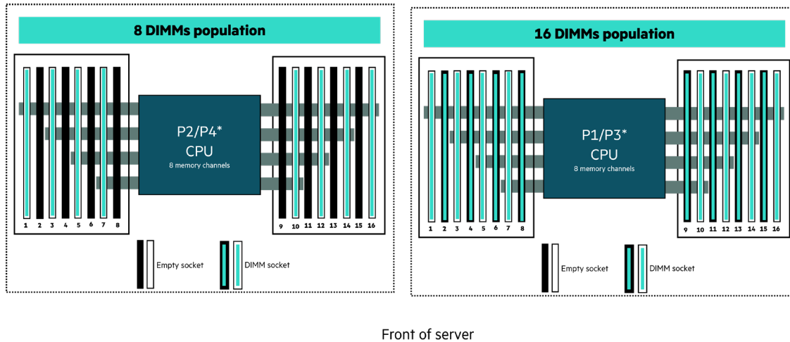
Figure 6. DIMM slot locations in HPE ProLiant DL360/DL380/ML350/DL560 Gen11 (5th Intel Xeon) Servers
