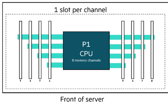
Figure 10. DIMM slot locations in HPE DL110 Gen11 (5th Intel Xeon) Servers (MLB is rotated compared to HPE DL360/DL380.)
