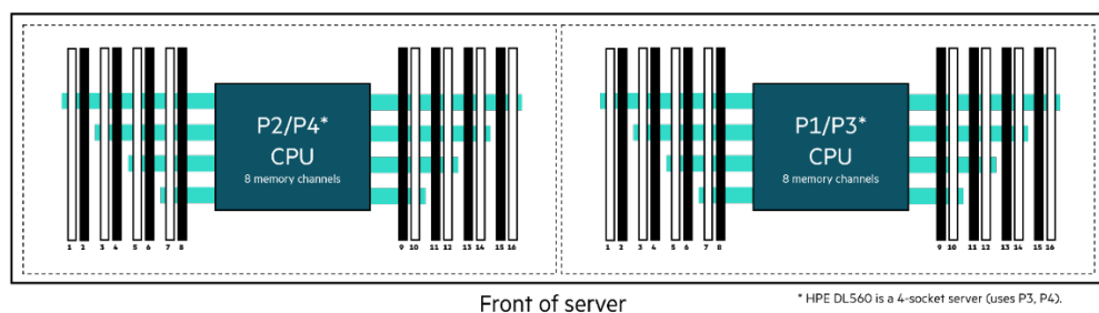
Figure 1. 32 DIMM slot locations in HPE ProLiant DL360/DL380/ML350 and 64 DIMM slot locations in HPE DL560 Gen11 (5th Intel Xeon) Servers
