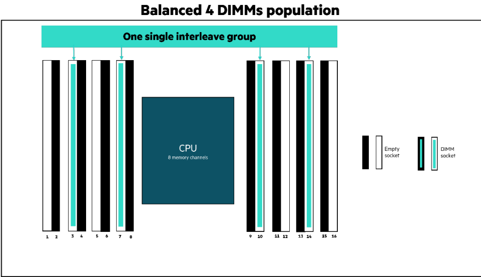
Figure 2. Example of memory that has balanced population
