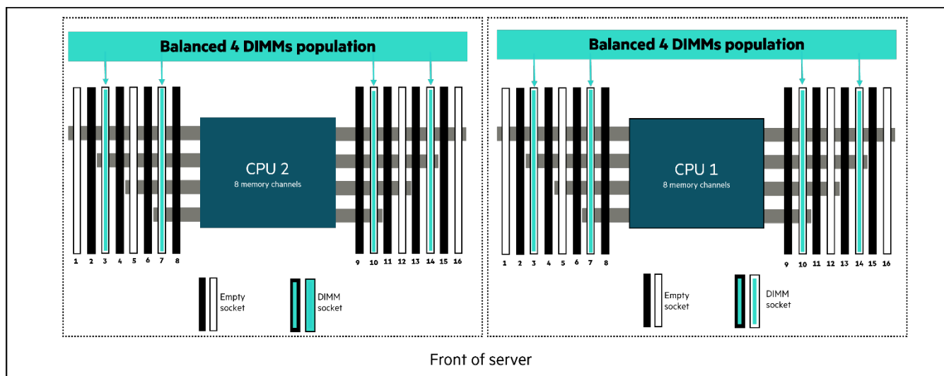
Figure 5. Example of a memory configuration that is balanced across processors
